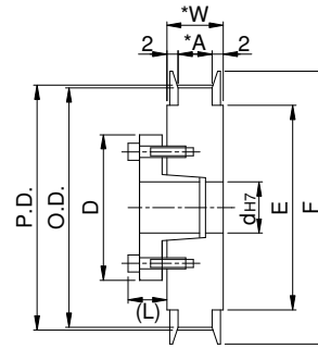
Pulley Shapes : E
