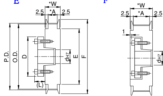
Pulley Shapes :
