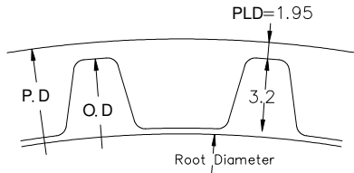
Tooth Shape :
