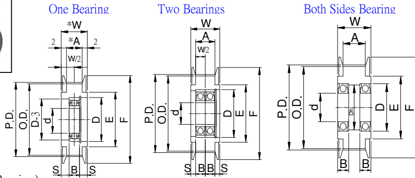
Pulley Shapes :
