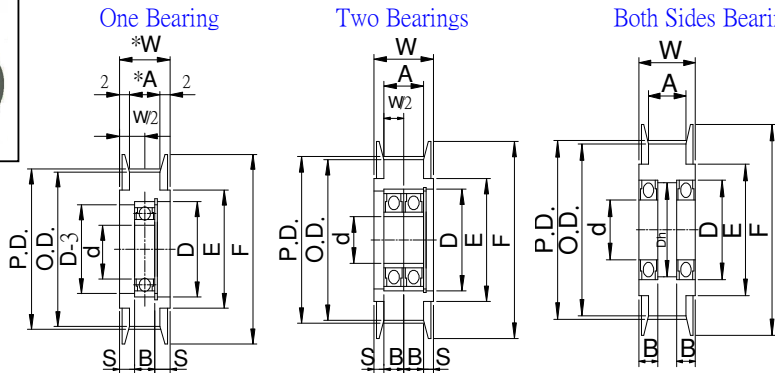
▲AT10 (Central Bearing)
