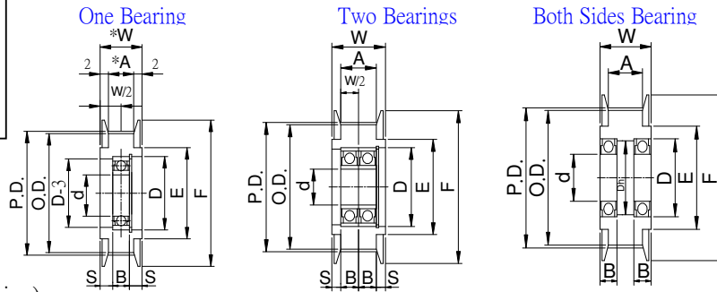
Pulley Shapes :
