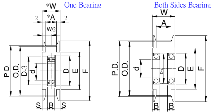
Pulley Shapes :
