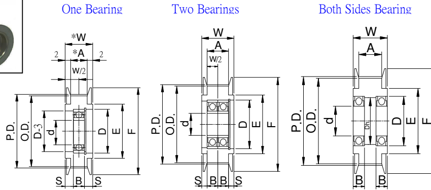
Pulley Shapes :
