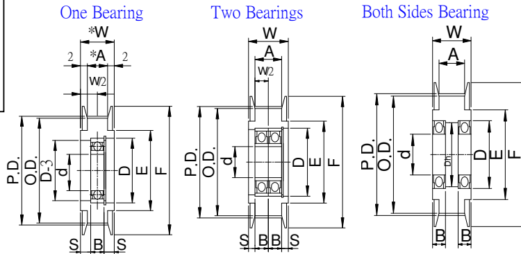
Pulley Shapes :
