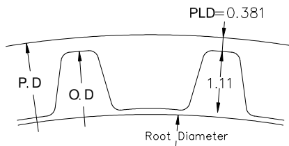
Tooth Shape :
