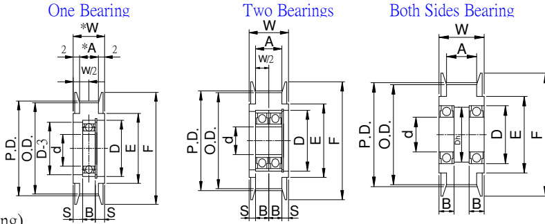
Pulley Shapes :
