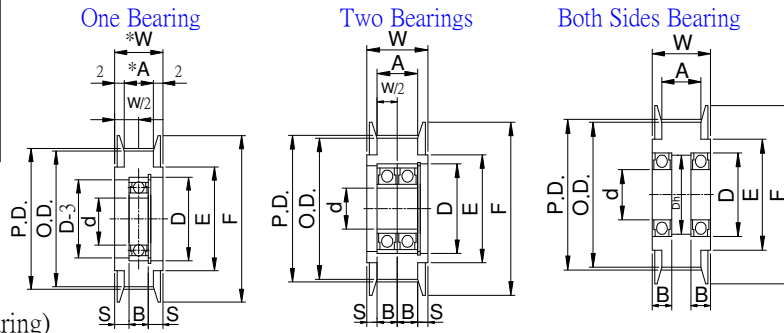
Pulley Shapes :
